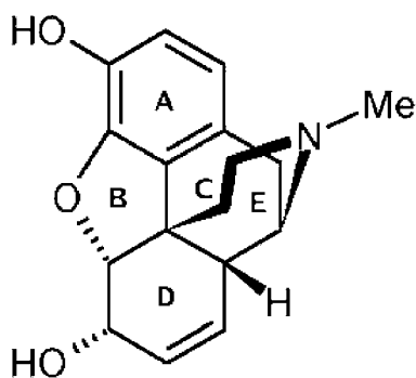
Figure 2 Definition of the rings in the oligocyclic structure of morphine.
